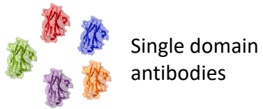
Recombinant proteins
